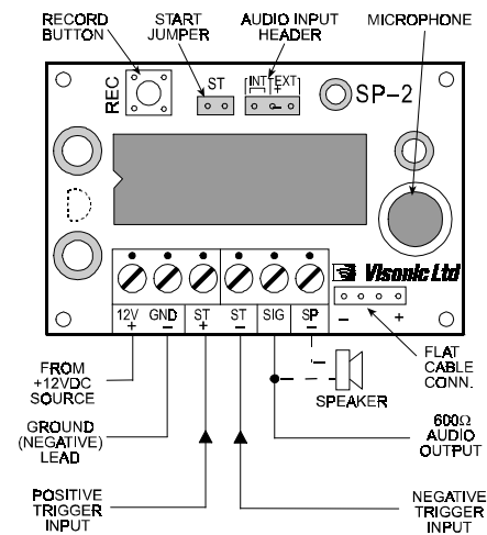
Figure 1. SP-2 module
