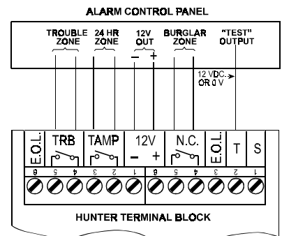
Figure 6. Terminal Block Wiring
