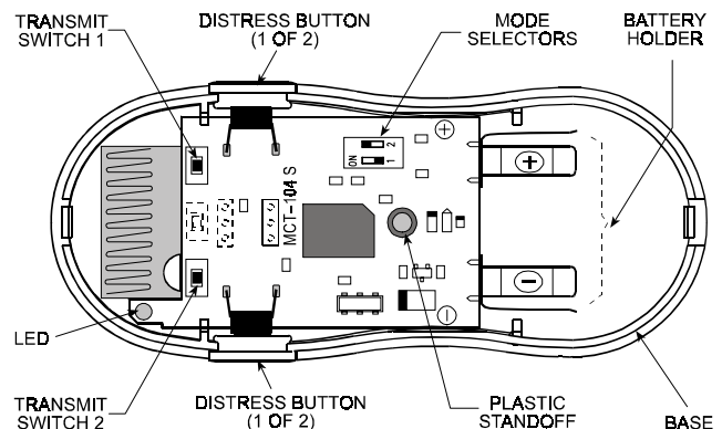
Figure 3. Component Layout
