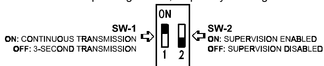
Figure 4. Mode Switch Tasks and Positions
