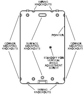
Figure 3. Knockout Locations
