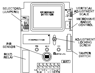
Figure 2. Printed Circuit Board
