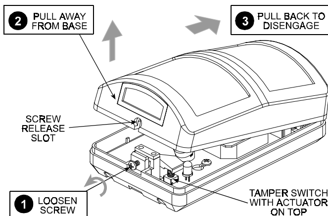
Figure 3. Cover Removal
