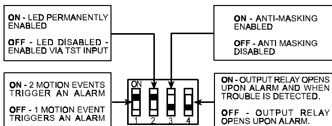
Figure 7. DIP Switch Mode Selector
