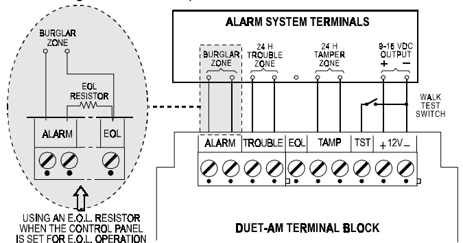
Figure 6. Terminal Block Wiring
