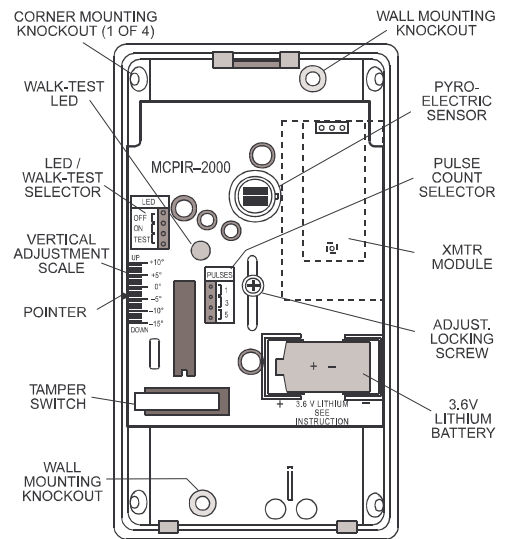
Figure 7. Components Layout
